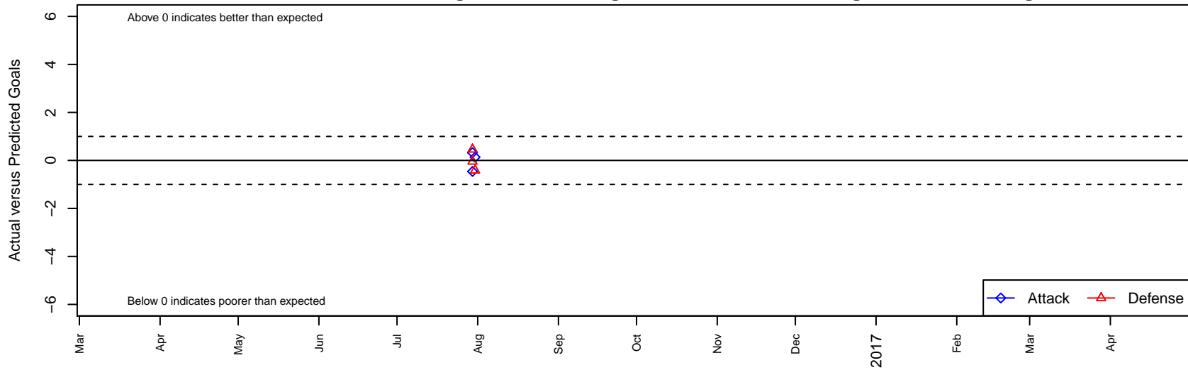
CDA Slammers SC EGSL Salazar G02 Dots are actual minus expected GF (blue circles) and GA (red triangles). Blue line is smoothed change in attack strength. Red is smoothed change in defense strength.
